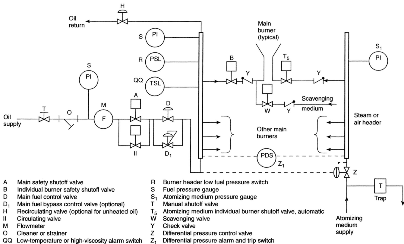
Typical Steam or Air Atomizing Main Oil Burner System
