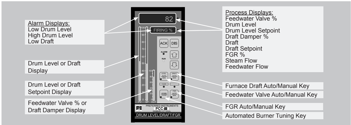
BurnerMate Model BM-AC Front Panel
