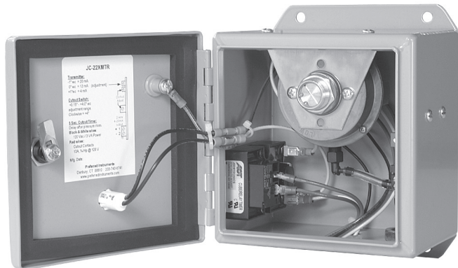
Draft Range Transmitter Assembly with Model JC-22XMTR (with door shown open)
